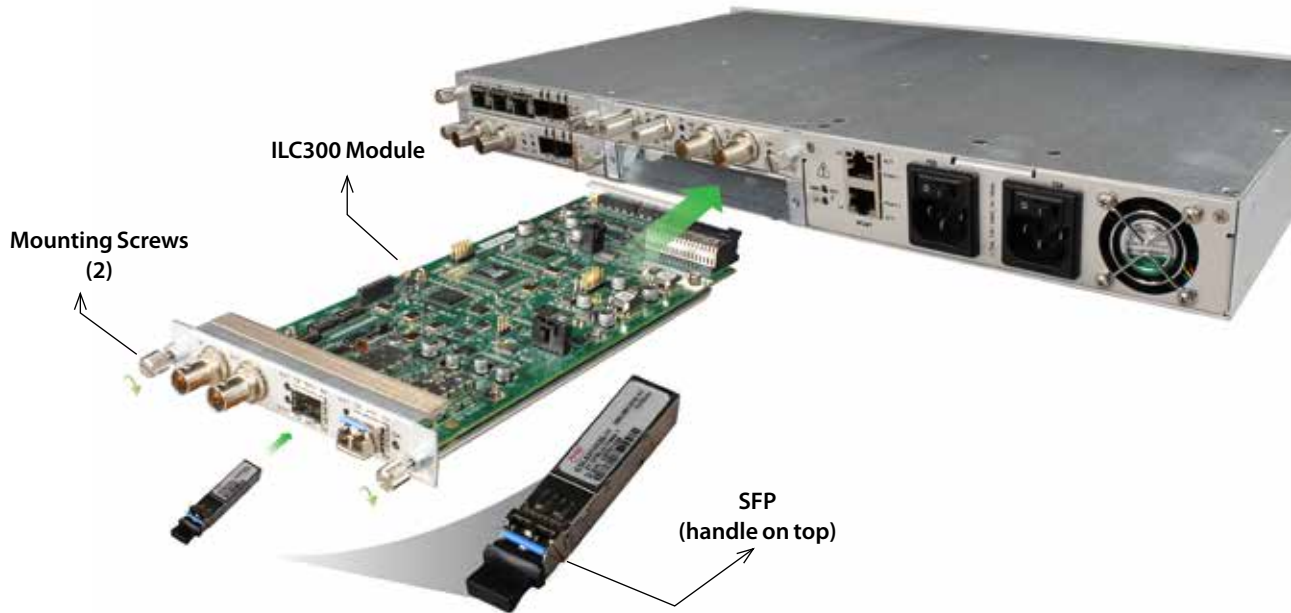
Figure 5. ILC300 Module and SFP Installation
