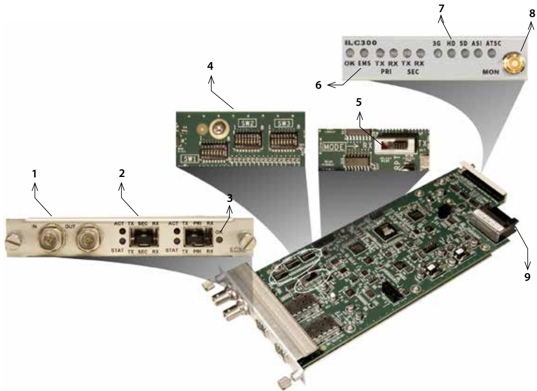
Figure 2. ILC300 Module Major Components
