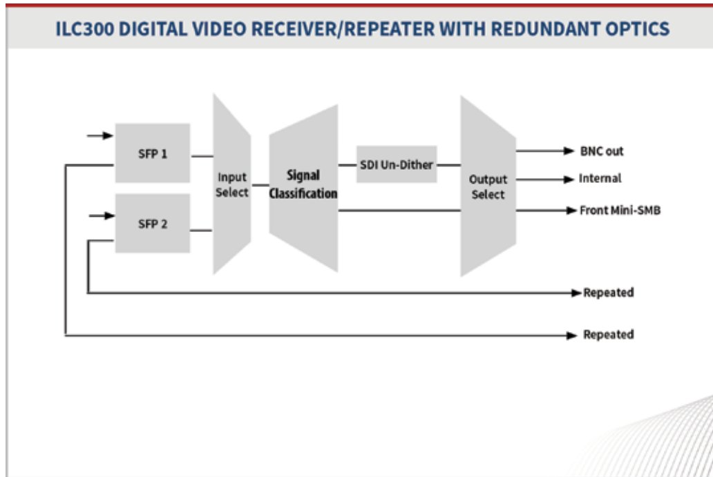
Figure 1. ILC300 Module Functional Block Diagram
